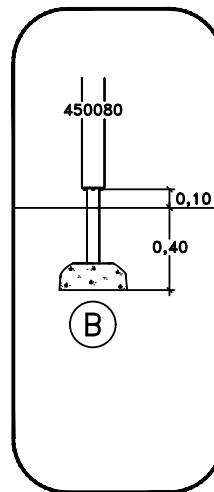
Sunken Foundation
